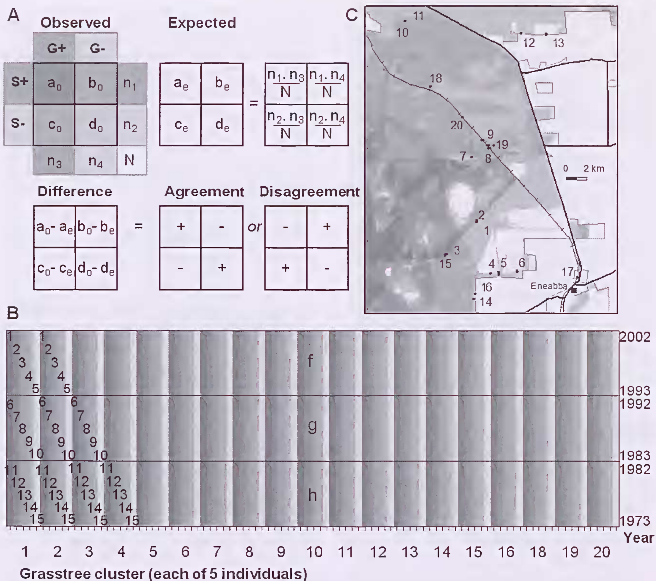
Figure 3 The Ward (2009) approach to assessing agreement among the grasstree and satellite records. (A) Counts of fire presence (+) and absence (-) observed in the grasstree G and satellite S records were tabulated in a two-way table. The difference between these observed ( o ) and expected ( e ) counts, calculated from marginal totals ( n ), indicates whether there is more agreement ( a + d ) or disagreement ( b + c ) than expected for the table. (B) To create more tables, the data were divided into three decades (f, g, h), each with 95 individual grasstrees sampled (vertical grey bars; the grasstrees were arranged in 20 clusters of 5 individuals: Ward excluded the 17th cluster as it had neither more nor less agreement). These decadal data were then further divided longitudinally, with one single individual from each cluster per group. This creates 15 tables (here numbered diagonally), where 1 = the 1st grasstree in each cluster in the 1st decade, 2 = the 2nd grasstree in each cluster in the 1st decade ... to 15 = the 5th grasstree in each cluster in the 3rd decade. (C) The spatial distribution of the 20 grasstree clusters around the Eneabba sandplain, overlain on the satellite fire history (dark shades indicate more fires).
